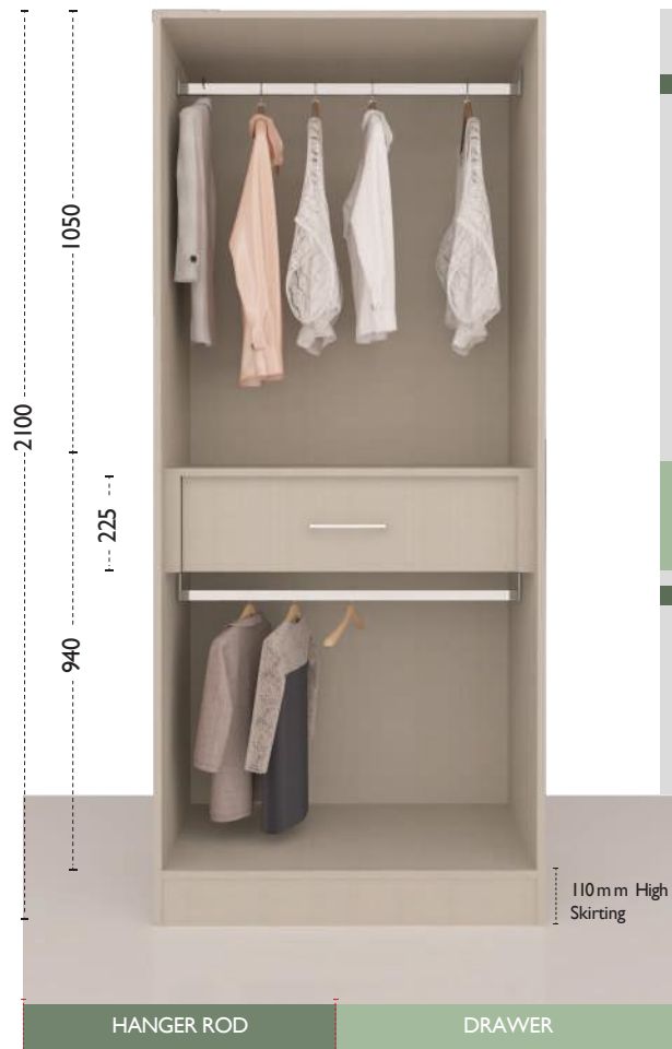
Double Shutter Unit (601 - 900)mm
