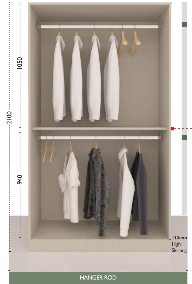
Double Shutter Unit (901 - 1200)mm
